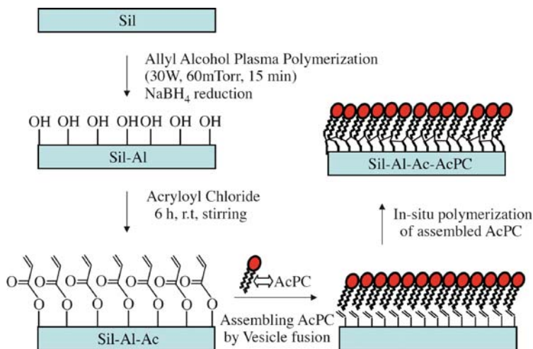
Fig. 3 Schematic illustration of the procedure for chemically grafting a polymerized lipid monolayer onto a silicon catheter surface. Reprinted with permission from [60]. Copyright 2005, Elsevier
