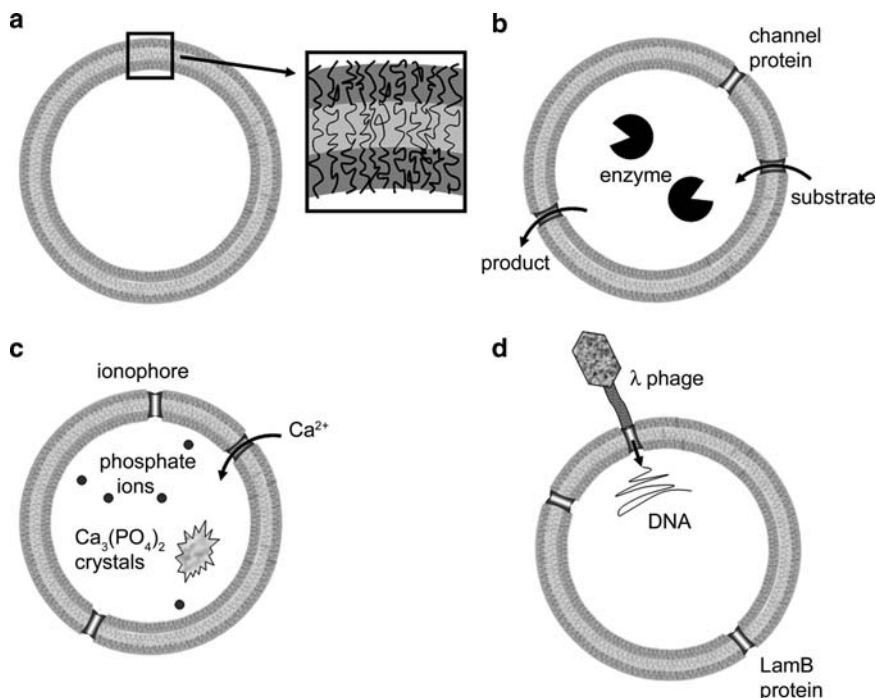
Fig. 16 a–d Schematic representation of polymer nanoreactors. a Cross section of triblock copolymer vesicle. b Polymersome with encapsulated enzyme and membrane-embedded channel protein. In the case described in the text, the substrate entering the vesicle is ampicillin, and the product of the hydrolysis is ampicillinoic acid. c Polymersome with embedded ionophores allowing \text{Ca}^{2+} ions to enter the vesicle where they react with phosphate ions to form calcium phosphate crystals. d The LamB protein serves as a receptor to the \lambda phage virus which can inject its DNA through the channel into the polymersome [259]. Reproduced with permission of The Royal Society of Chemistry
