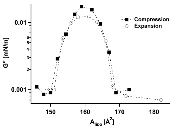
Fig. 21 Loss modulus vs A_{lipo} plotted for 40% lipopolymer during compression and expansion of bilayer shows reversibility of the viscoelastic transition. Also, the gel exhibits a collapse at smaller A_{lipo} (and higher pressures) than pure lipopolymer [42] (reproduced with permission from the American Chemical Society)
